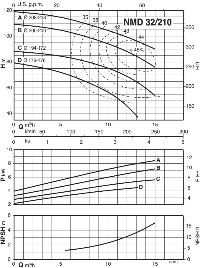
Characteristic curves n ≈ 2900 rpm
