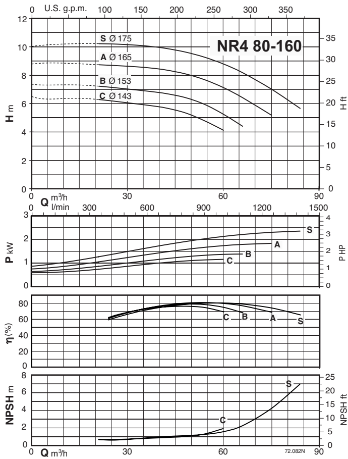
Coverage chart n \approx 1450 rpm
