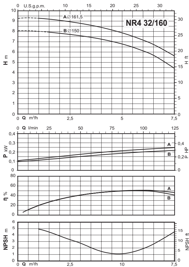
Coverage chart n \approx 1450 rpm
