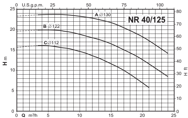
Coverage chart n \approx 2900 rpm
