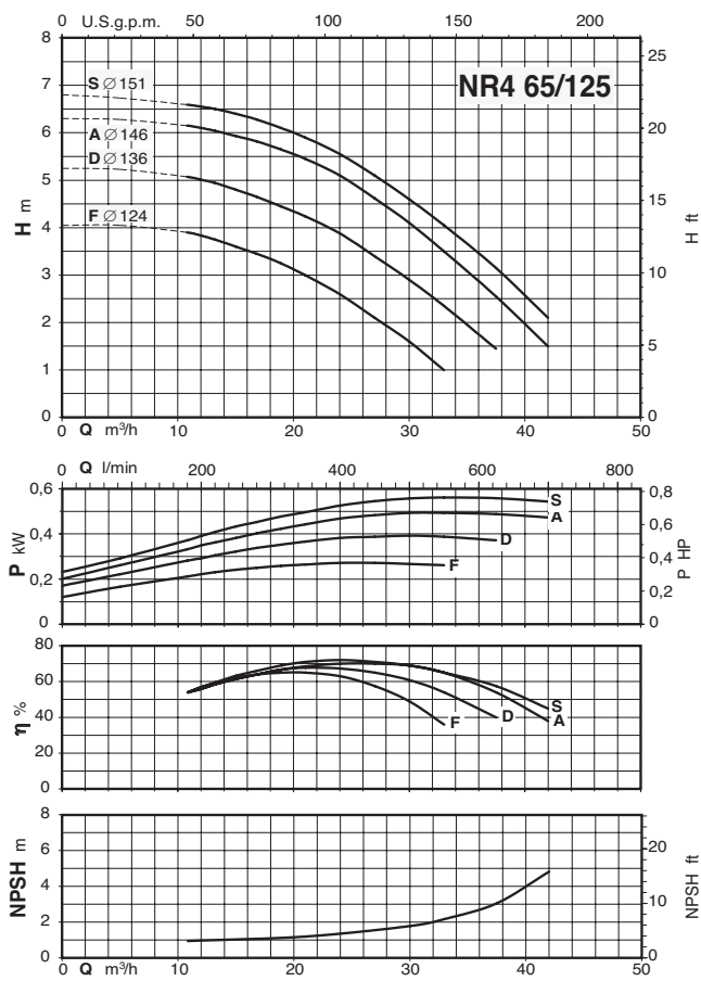
Coverage chart n \approx 1450 rpm
