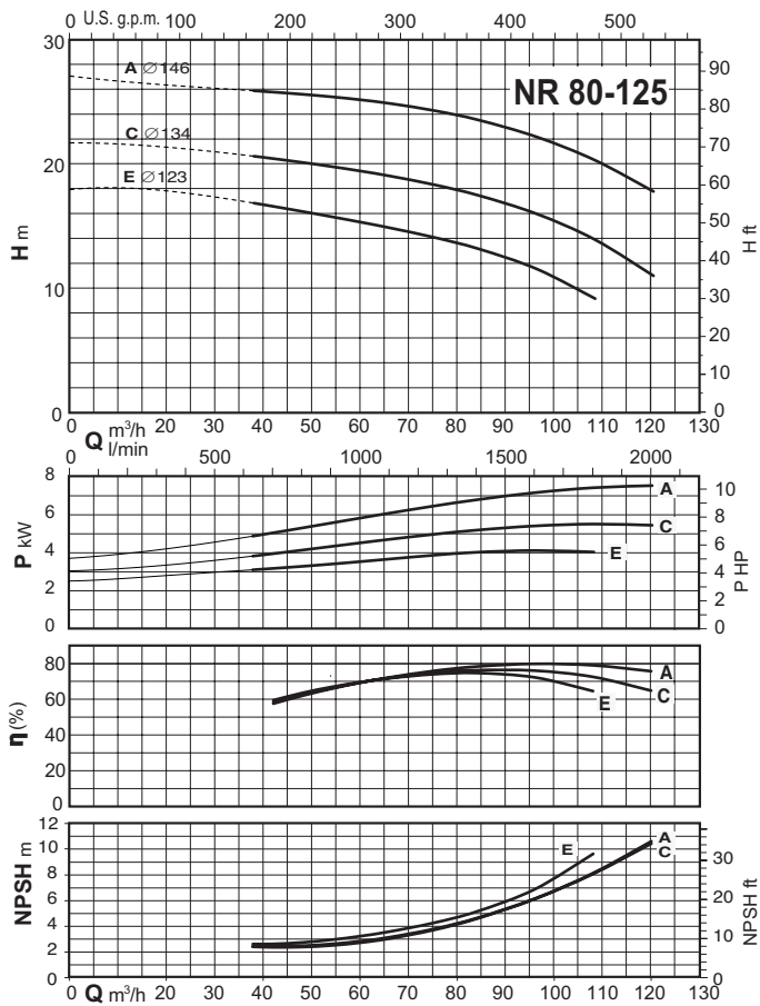
Coverage chart n \approx 2900 rpm
